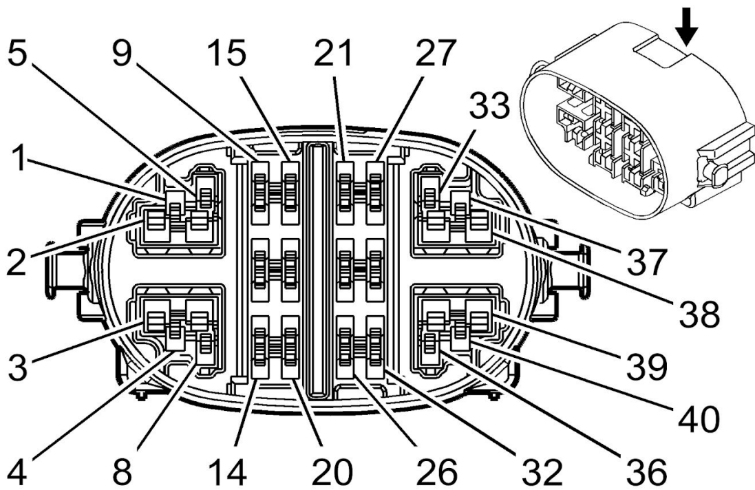
X108 Connector
