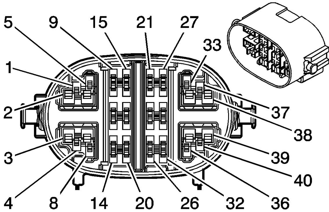
X107 Connector
